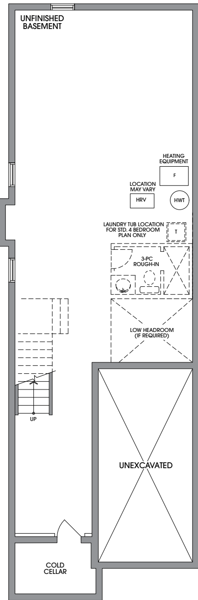
BASEMENT ELEVATION A & B
