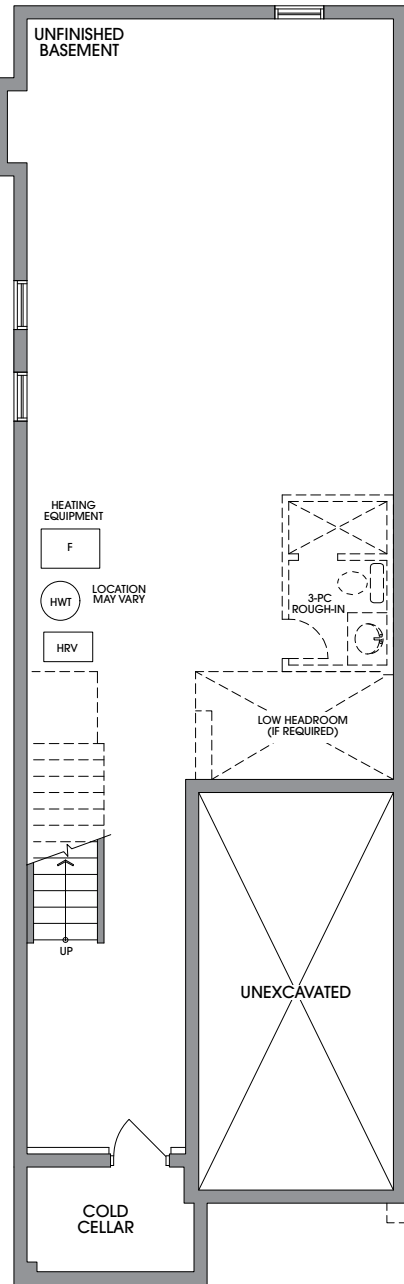
BASEMENT ELEVATION A & B
